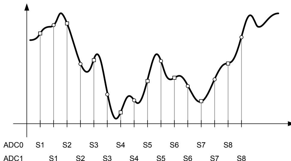
Figure 18-5. Skewed Sampling
