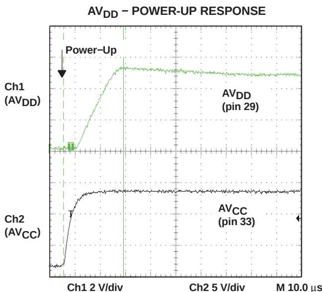
Figure 46. Power-Up Response
