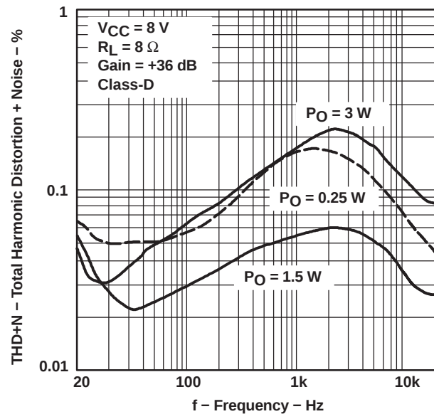
TOTAL HARMONIC DISTORTION + NOISE VS FREQUENCY
