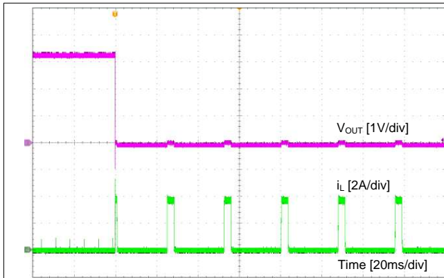
Figure 20. Short Protection
