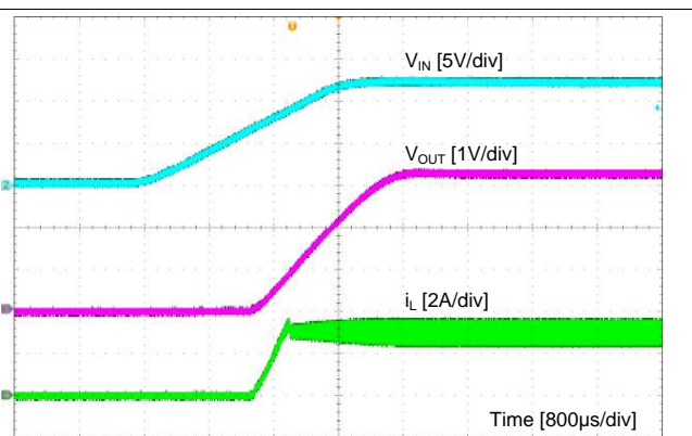
Figure 15. DCM Mode
