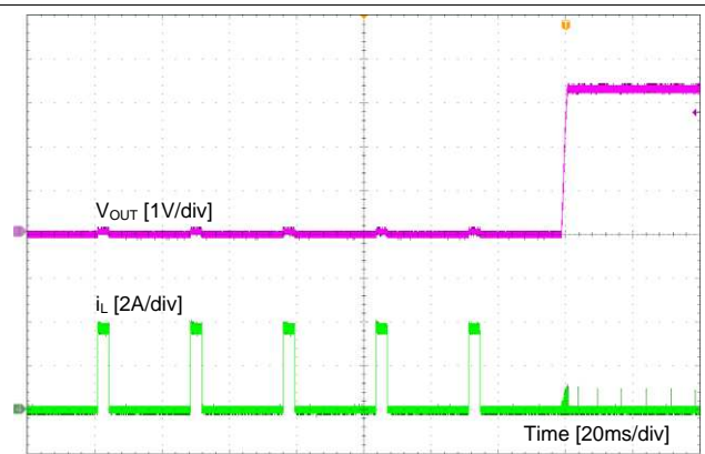
Figure 21. Short Recovery
