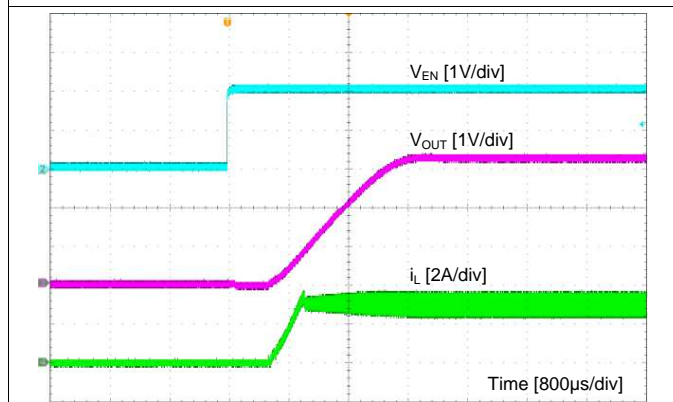
Figure 16. PSM Mode
