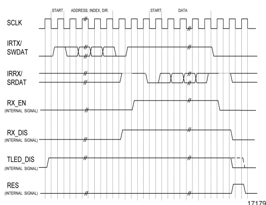
Figure 12. Read Data Waveform
