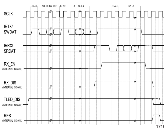
Figure 13. Read Data Waveform with Extended Index
