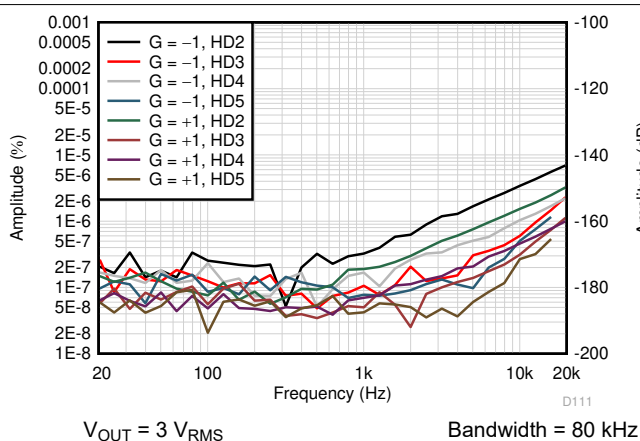
图 6-9. Individual Harmonic Amplitude vs Frequency
