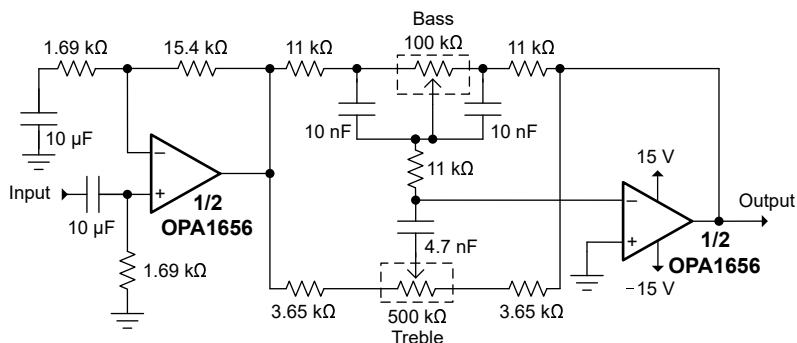
图 8-9. Dual Potentiometer Baxandall Tone Control
