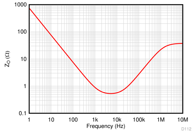
图 6-40. Open-Loop Output Impedance vs Frequency
