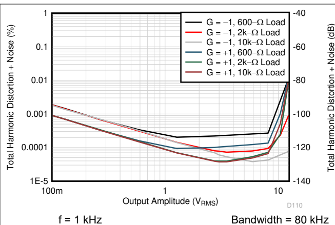
图 6-8. THD+N Ratio vs Output Amplitude
