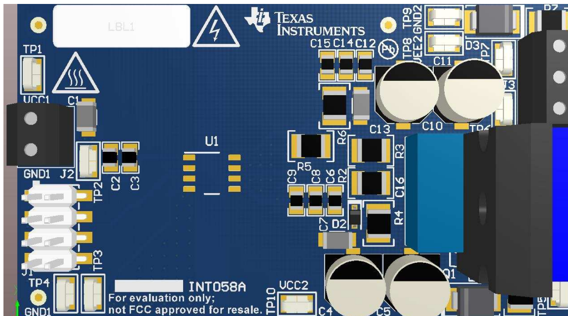
Figure 42. 3-D PCB View
