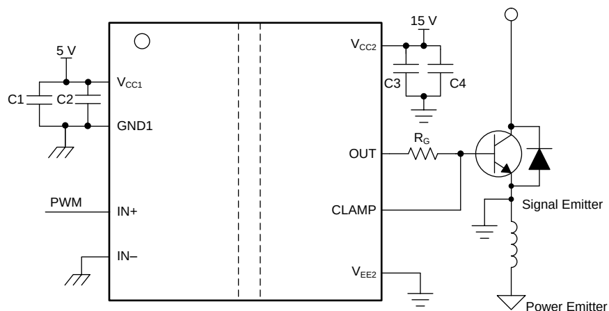
Figure 34. Typical Application Circuit for UCC5310M to Drive IGBT
