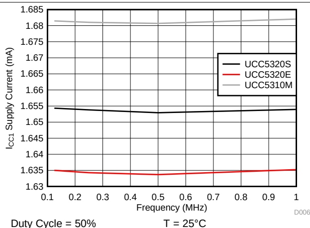
Figure 7. I_{CC1} Supply Current vs Input Frequency
