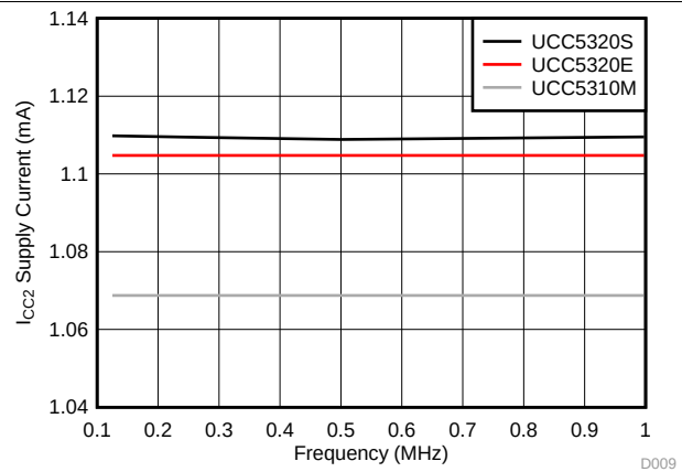
Figure 10. I_{CC2} Supply Current vs Input Frequency
