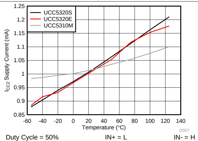
Figure 8. I_{CC2} Supply Current vs Temperature
