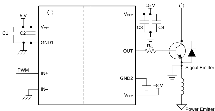
Figure 35. Typical Application Circuit for UCC5320E to Drive IGBT
