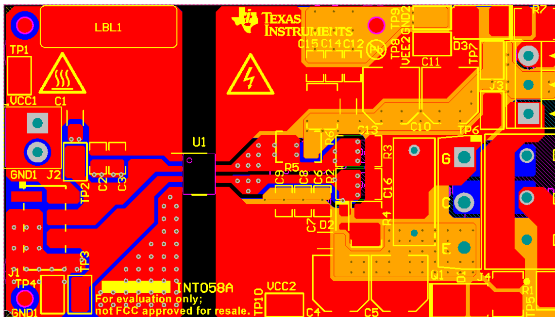
Figure 39. Layout Example
