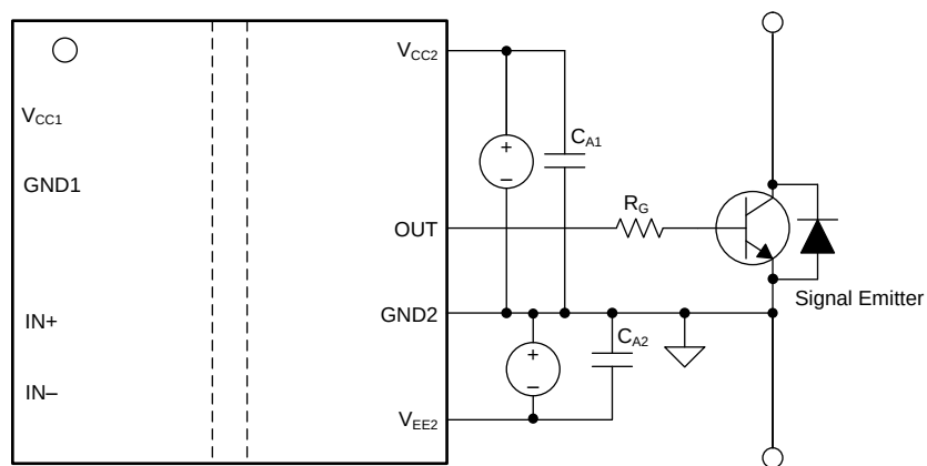
Figure 37. Negative Bias With Two Iso-Bias Power Supplies (UCC5320E)
