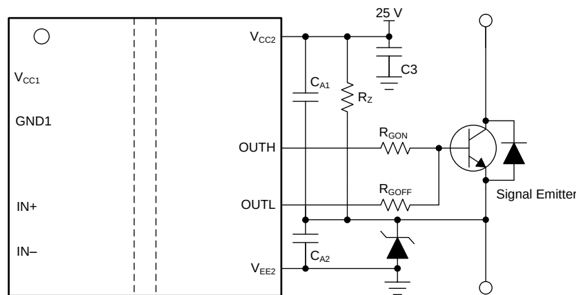
Figure 36. Negative Bias With Zener Diode on Iso-Bias Power-Supply Output (UCC5320S)
