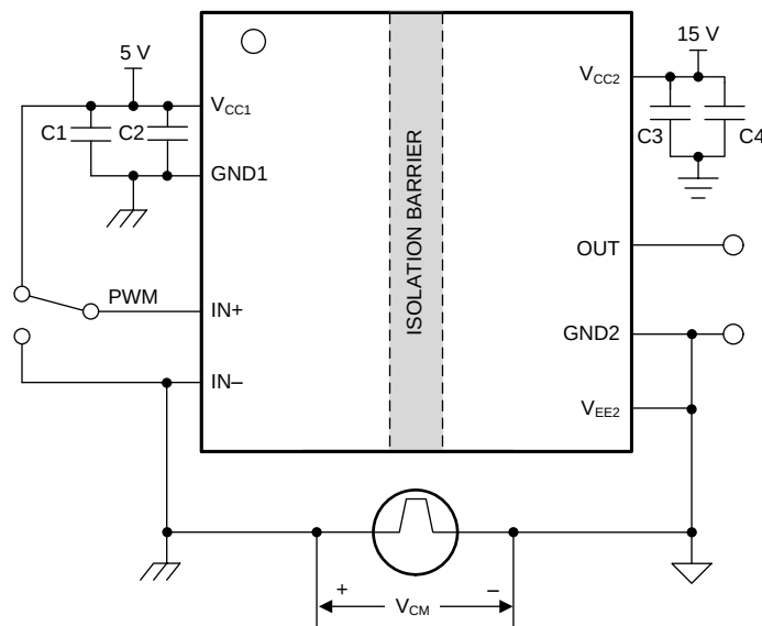
Figure 20. CMTI Test Circuit for UCC5320E
