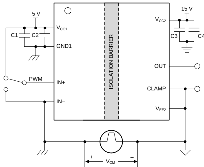
Figure 19. CMTI Test Circuit for UCC5310M
