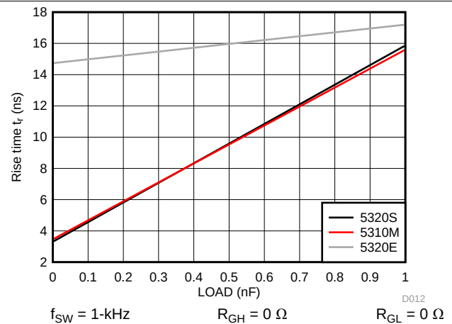
Figure 12. Rise Time vs Load Capacitance
