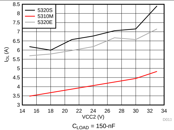
Figure 4. Output-Low Drive Current vs Output Voltage
