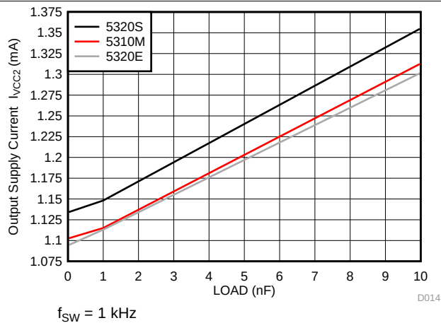
Figure 11. I_{CC2} Supply Current vs Load Capacitance
