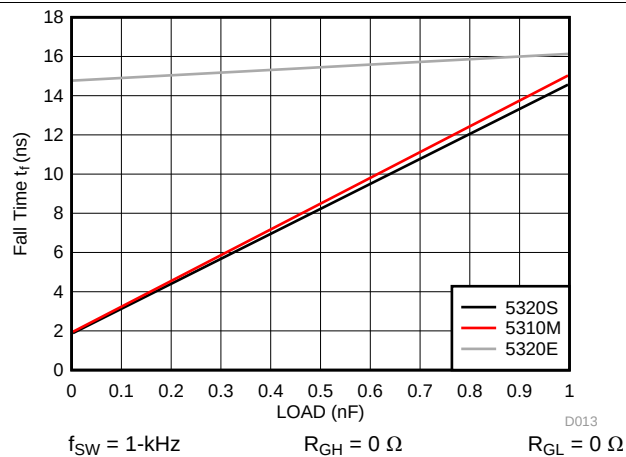
Figure 13. Fall Time vs Load Capacitance
