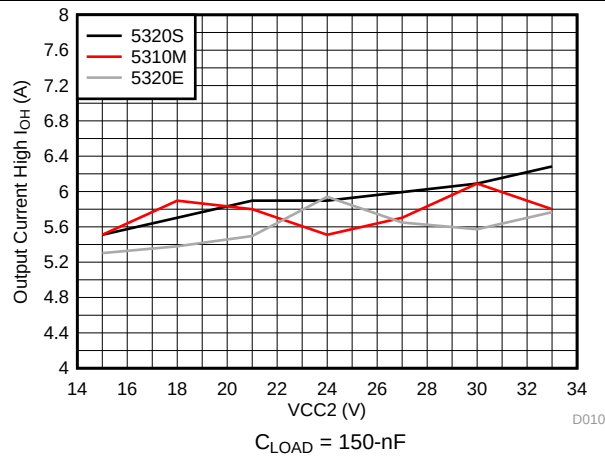
Figure 3. Output-High Drive Current vs Output Voltage
