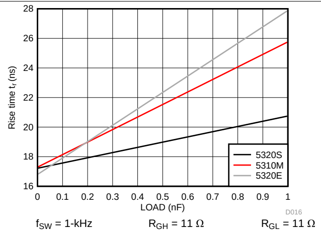
Figure 14. Rise Time vs Load Capacitance
