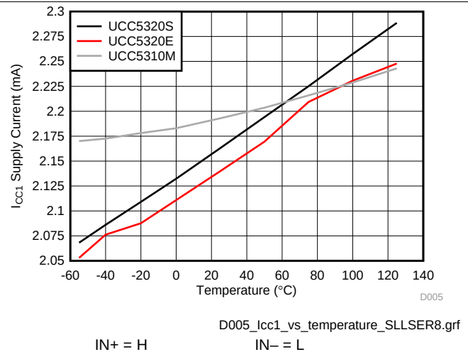
Figure 6. I_{CC1} Supply Current vs Temperature
