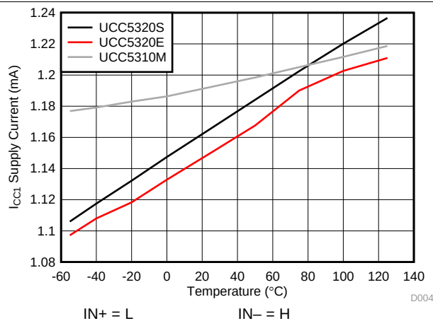
Figure 5. I_{CC1} Supply Current vs Temperature
