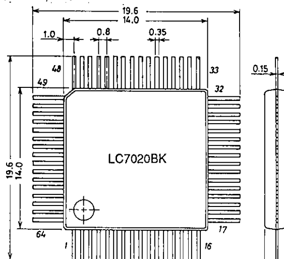
Package Dimensions 3026B-Q64BIC (unit: mm)
