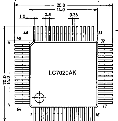
Package Dimensions 3057-Q64AIC (unit: mm)
