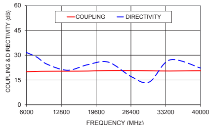
ZCDC20-K0644+ COUPLING & DIRECTIVITY
