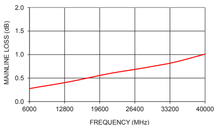
ZCDC20-K0644+ MAINLINE LOSS
