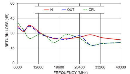
ZCDC20-K0644+ RETURN LOSS
