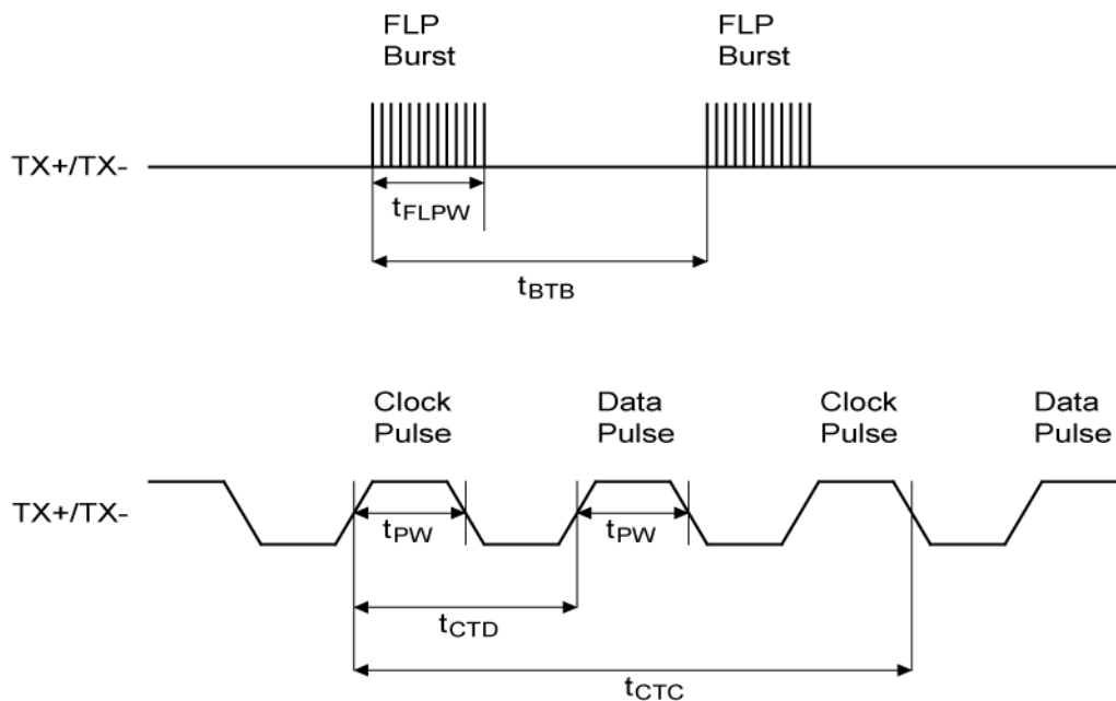
Figure 25: Auto-Negotiation Timing
