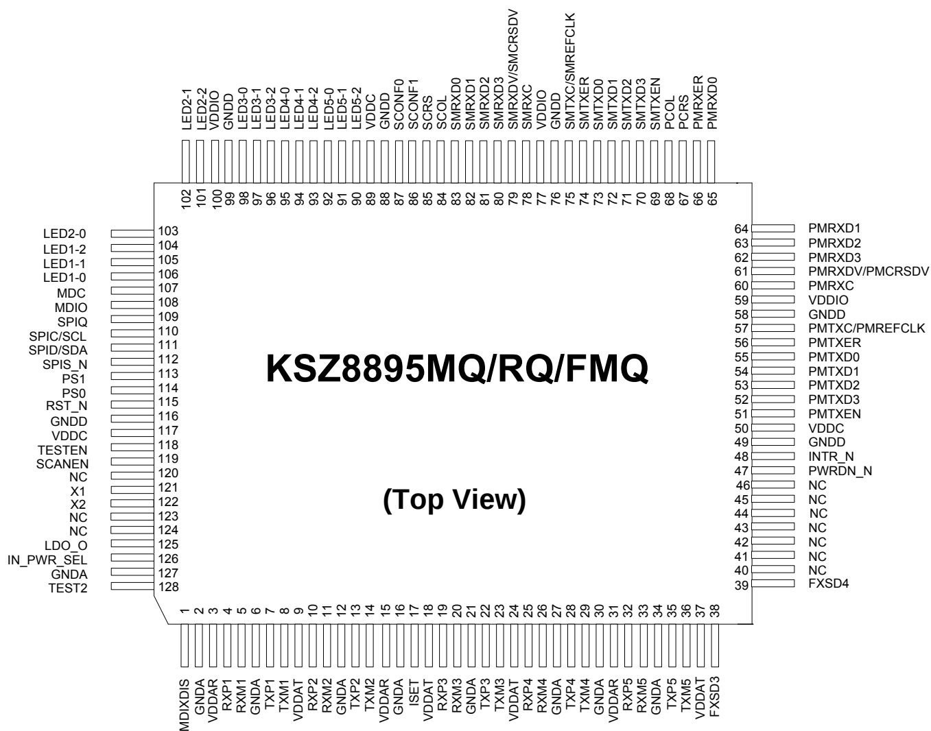
128-Pin PQFP
