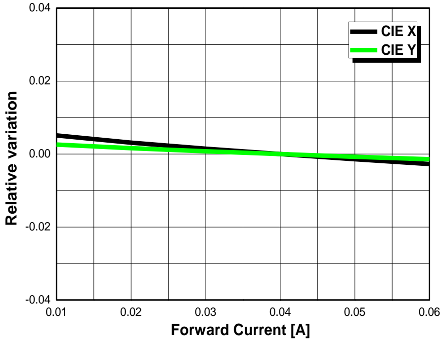
Fig 5. Forward Current vs. CIE X, Y Shift, T_a=25^\circ\text{C} (4200K~6000K)
