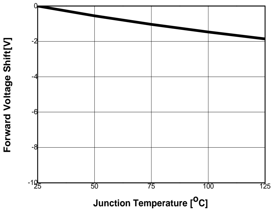
Fig 7. Junction Temperature vs. Relative Forward Voltage, I_F=40\text{mA}
