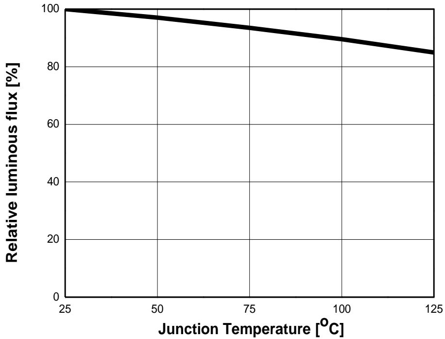
Fig 6. Junction Temperature vs. Relative Light Output, I_F=40\text{mA}
