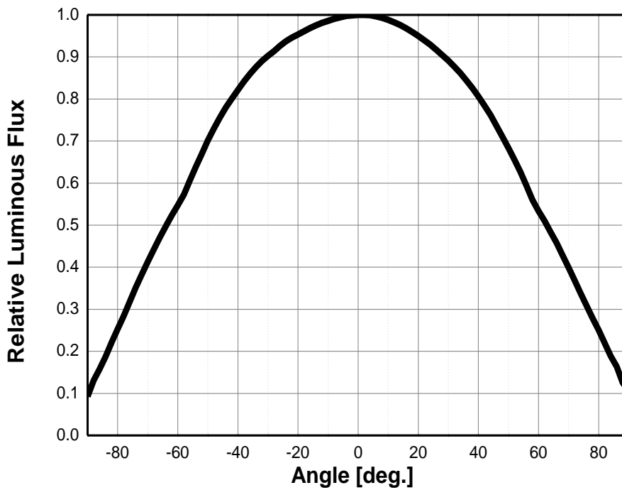
Fig 2. Viewing Angle Distribution, I_F=40\text{mA} , T_a=25^\circ\text{C}
