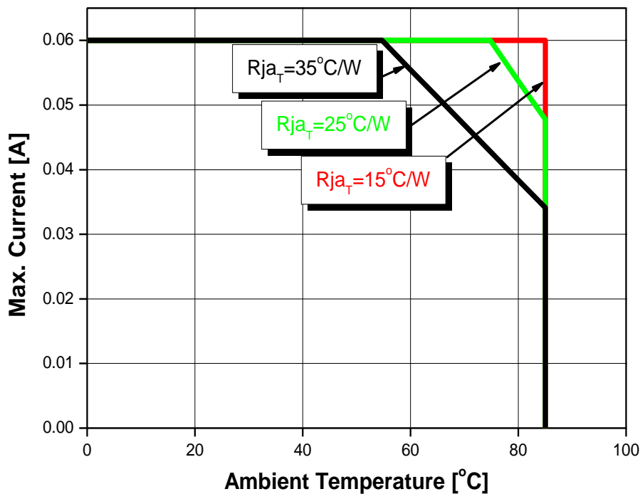
Fig 9. Maximum Forward Current vs. Ambient Temperature, T_j(max.)=125^\circ C , I_F=60mA
