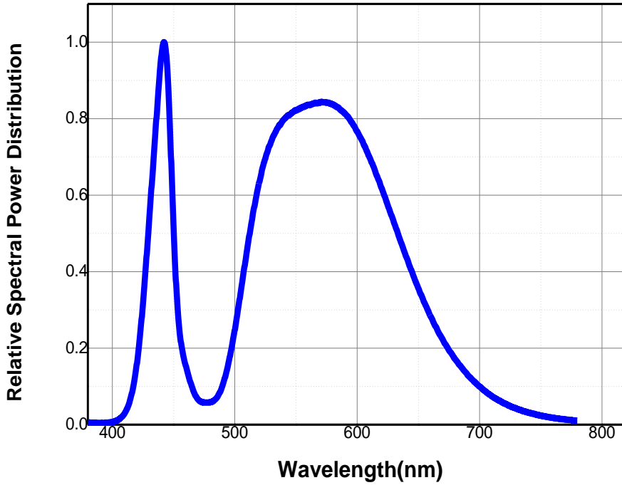
Fig 1. Color Spectrum, I_F=40\text{mA} , T_a=25^\circ\text{C} , RH30%
