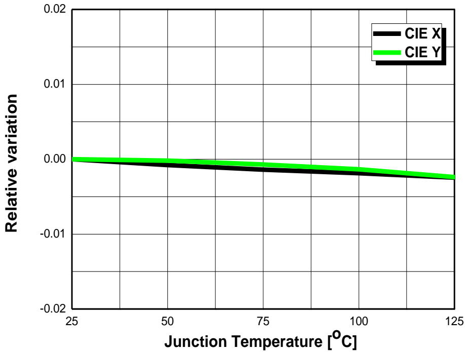
Fig 8. Junction Temperature vs. CIE x, y shift, I_F=40mA (4200K~6000K)
