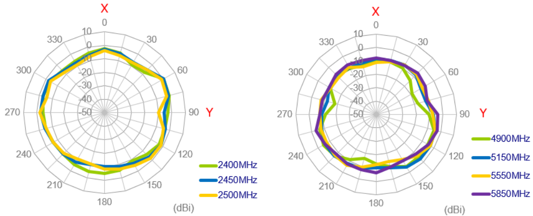
XZ Plane
