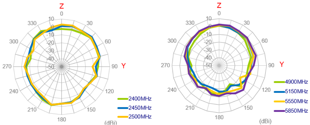
YZ Plane
