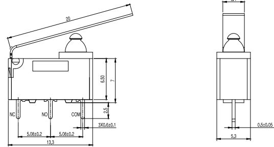
L20 LEAF LEVER WITH LENGTH 20 MM
