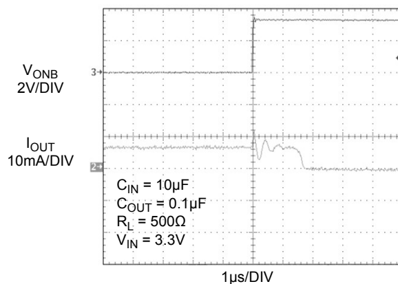
Figure 12. T_{OFF} Response
