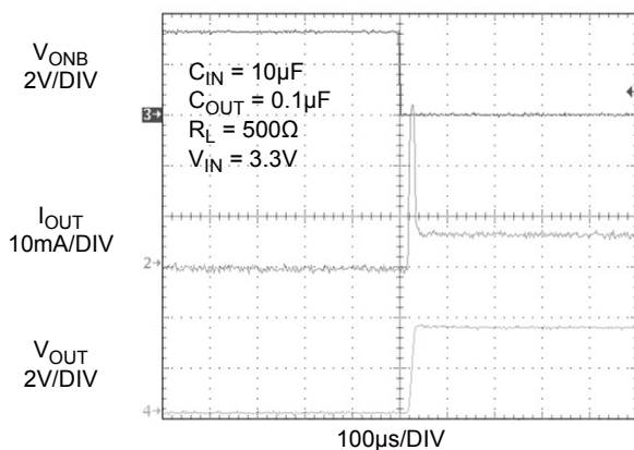
Figure 11. T_{ON} Response
