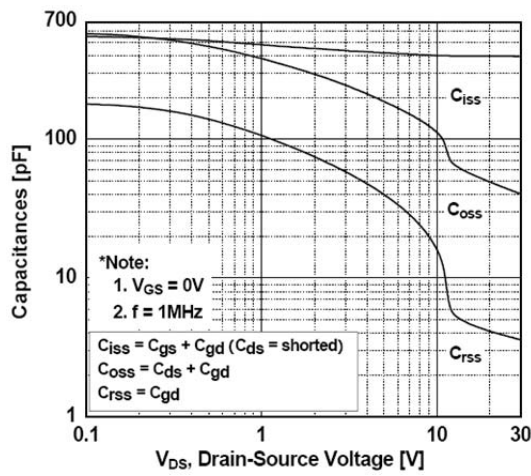
Fig. 5 Capacitance Characteristics
