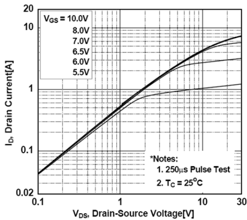
Fig. 1 On-State Characteristics
