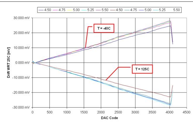
Figure 21. DAC2 Temperature Drift (mV)
