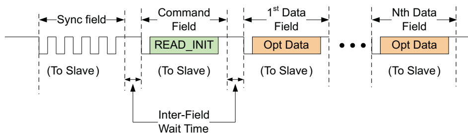
Figure 45. Read Initialization Frame
