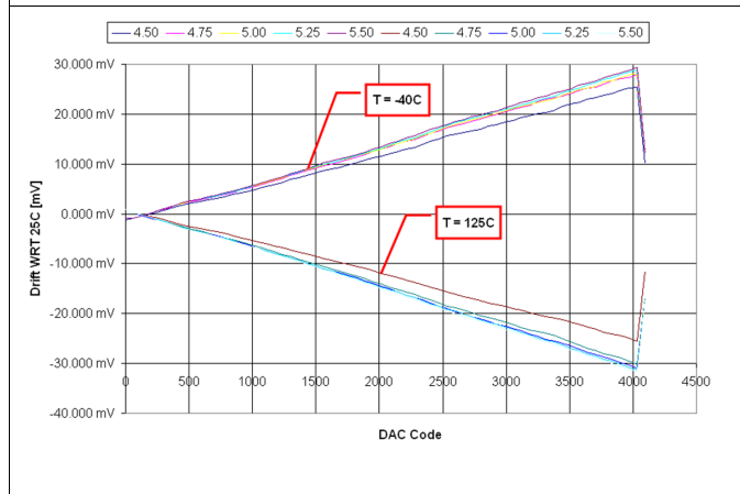
Figure 20. DAC1 Temperature Drift (mV)
