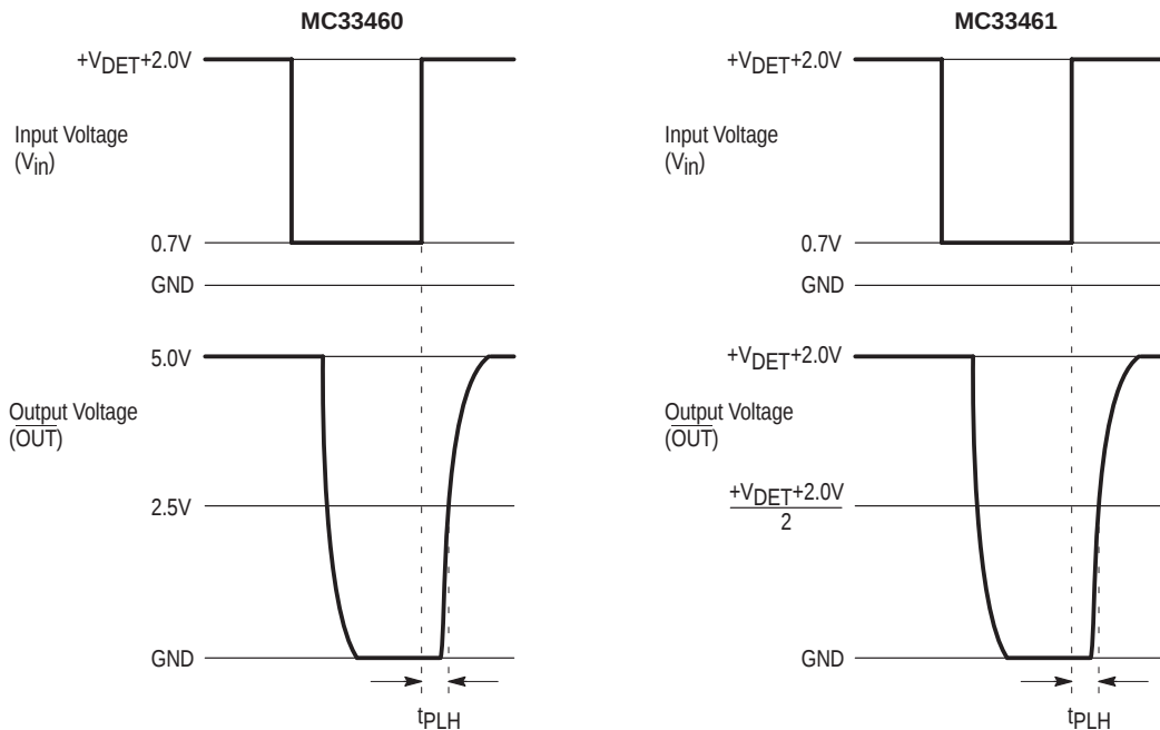
Figure 1. T_{pd} Measurement Conditions
