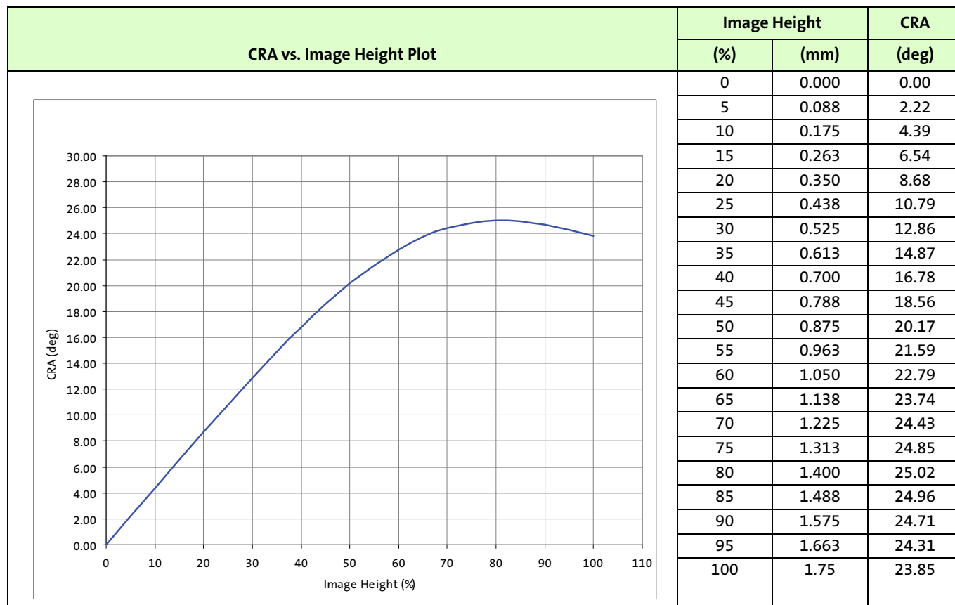
Figure 26: CRA vs. Image Height
