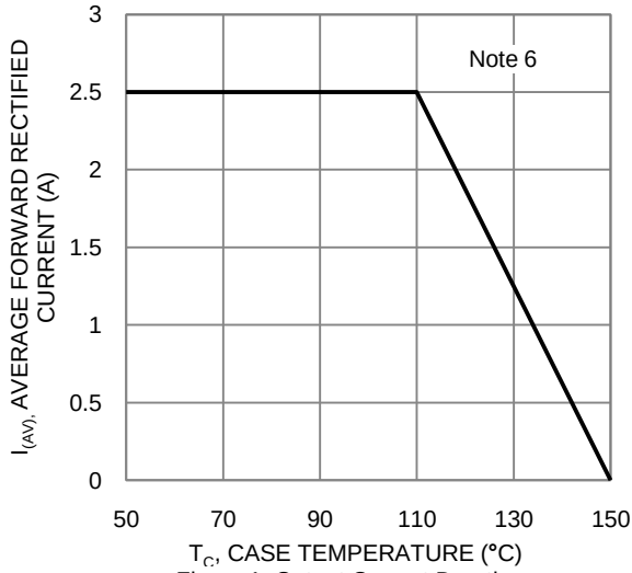
Figure 1. Output Current Derating Curve
