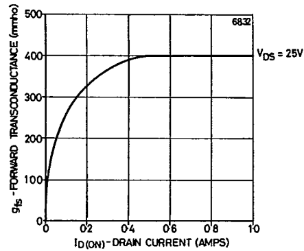
Fig. 7 Typical transconductance v drain current
