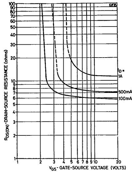
Fig. 5 Typical on-resistance v gate-source voltage
