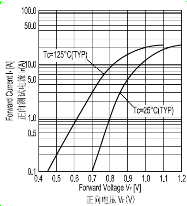
Fig3.Forward Voltage
