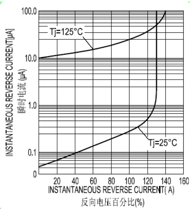
Fig2.Typical Reverse Characteristics
