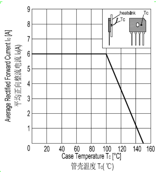
Fig1.Derating Curve
