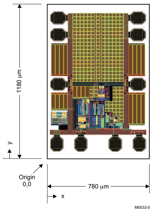
Figure 17. Chip Layout
