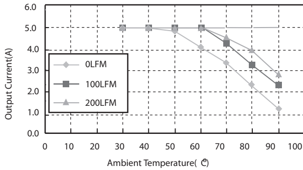
Figure 3. Typical Power De-rating for 12V IN 3.3Vout
