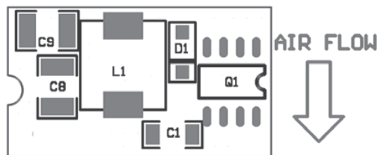
Figure 7. Temperature Measurement Location for VPOL5A-12-SMT
