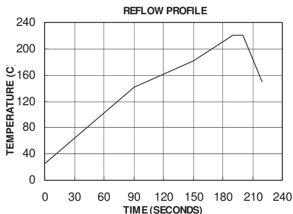
Figure 14 VPOL5A-12-SMT Reflow Profile
