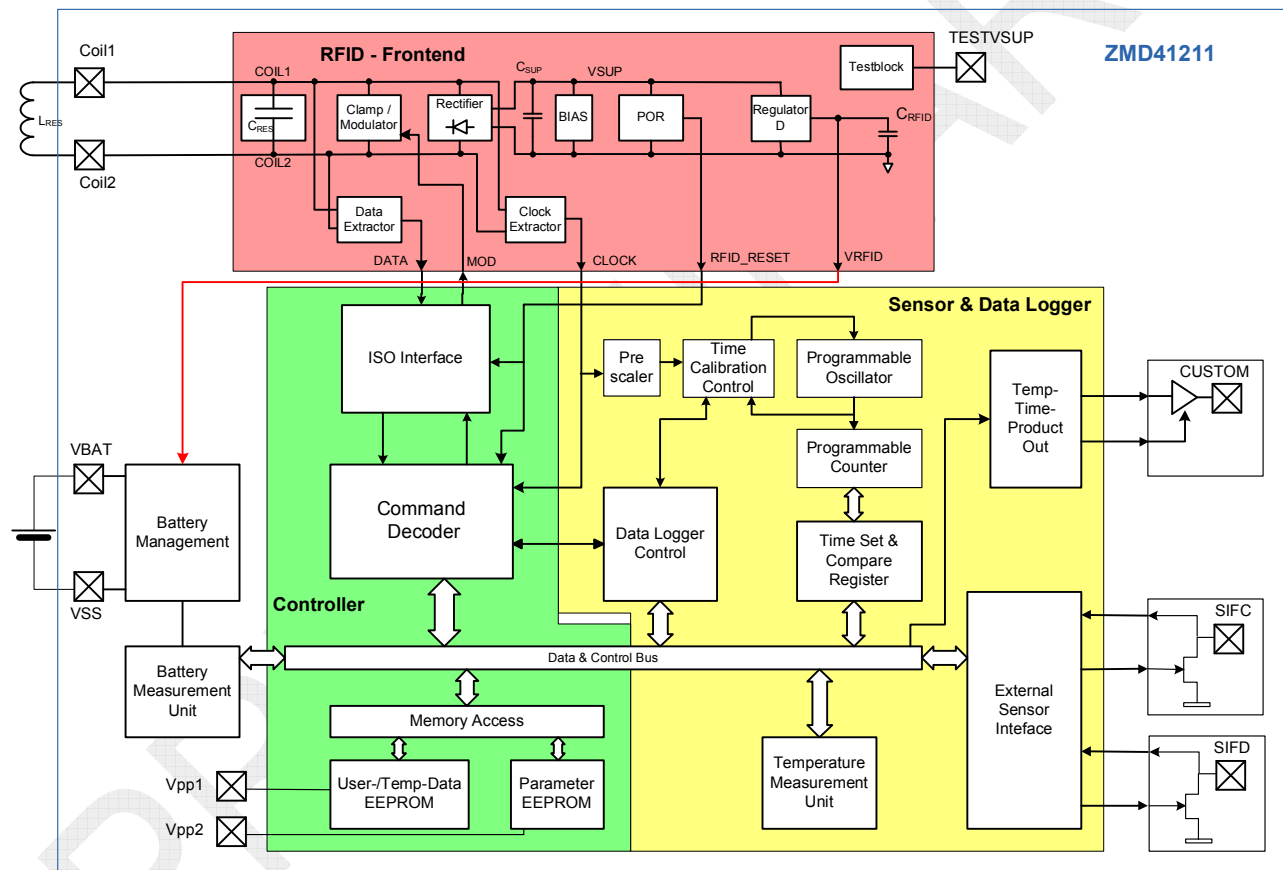
Figure 2.1 ZMD41211 Architecture
