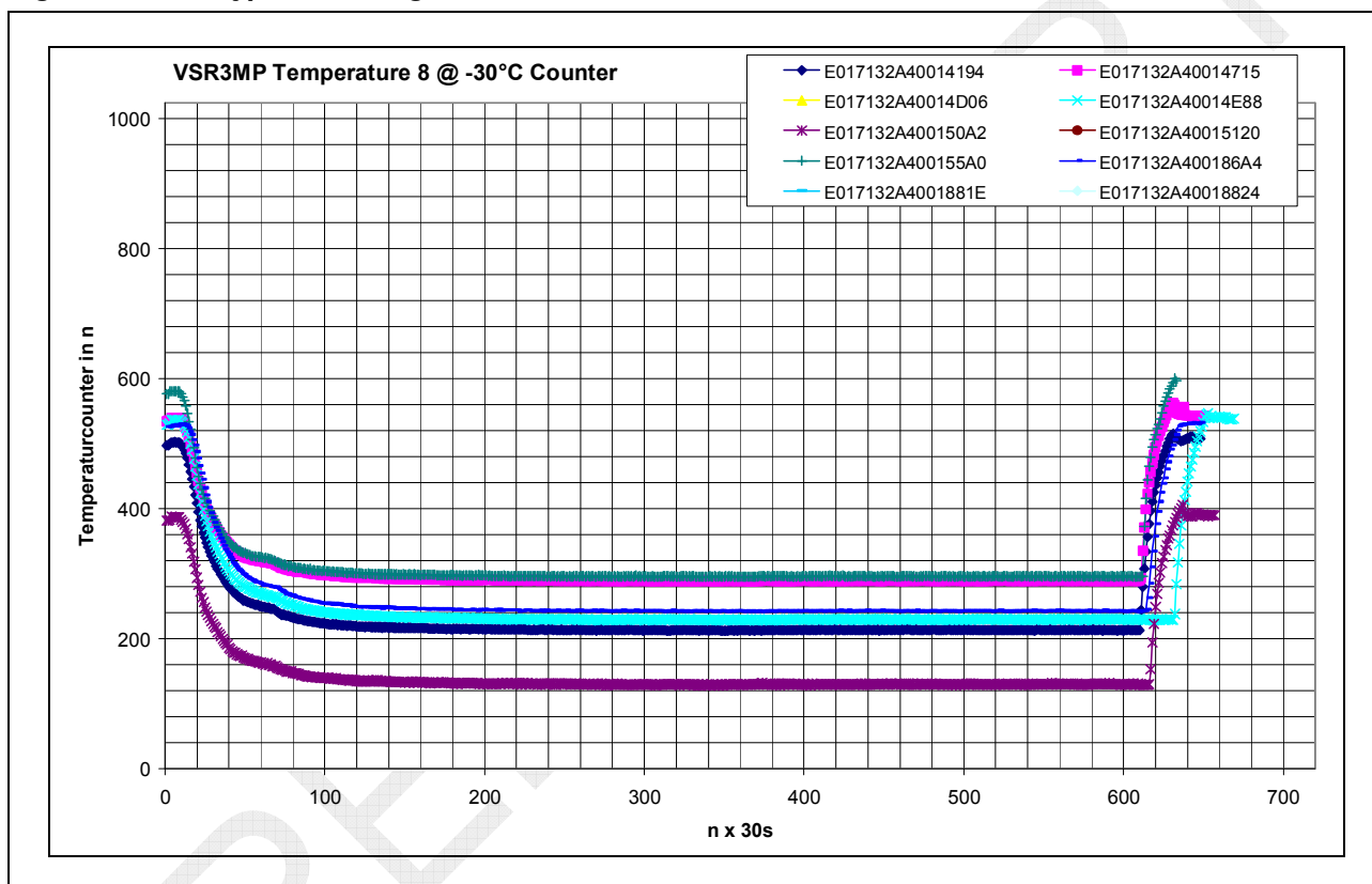
Figure 5.4 Typical Settling Behaviour
