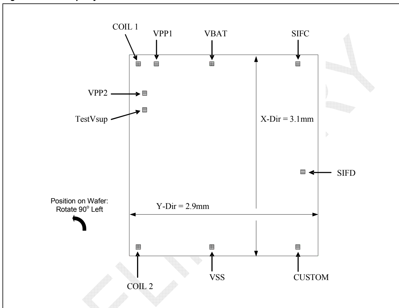
Figure 7.2 Chip Layout
