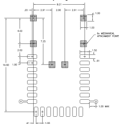
Footprint (PWB)
