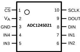
Figure 1. 10-Lead VSSOP See DGK Package
