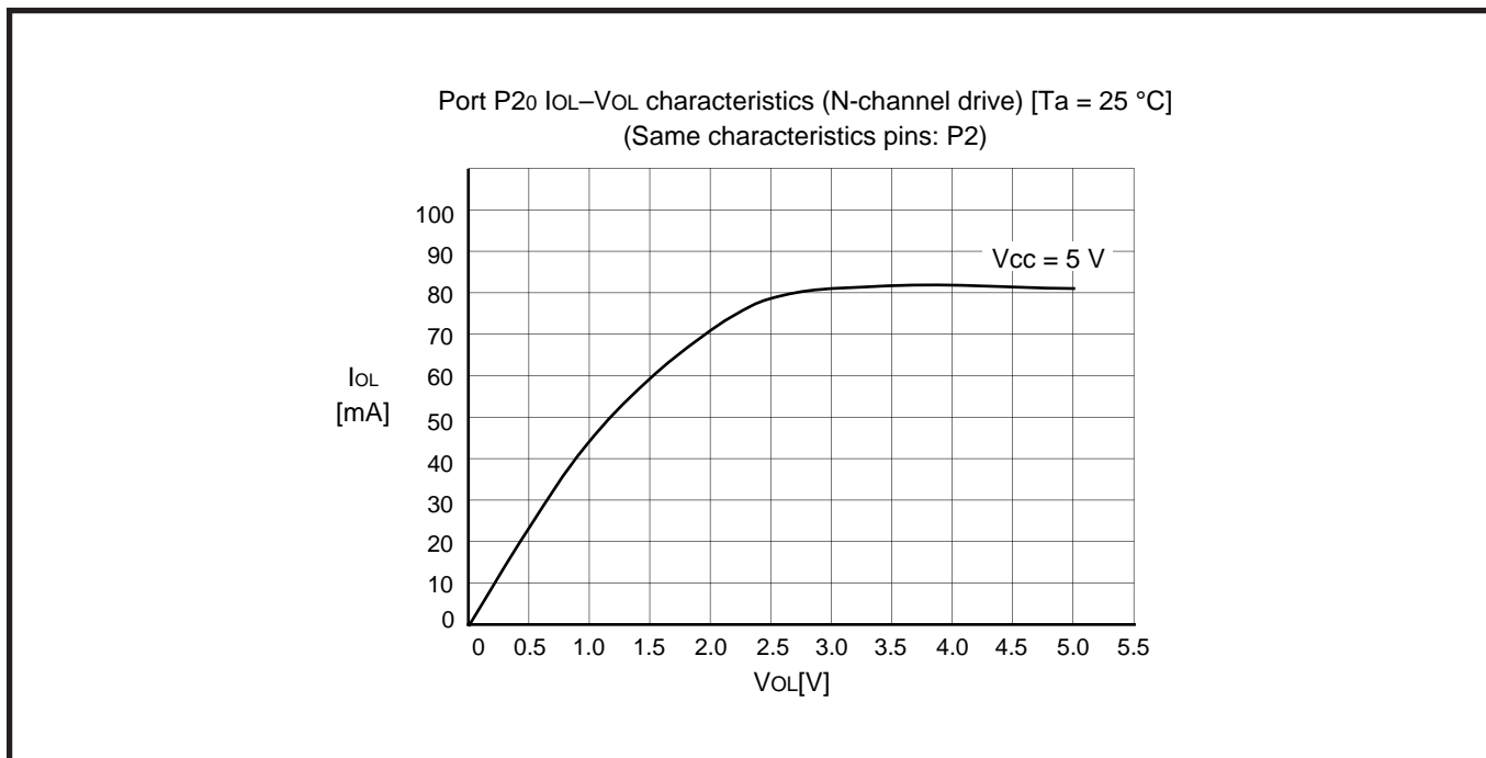
Fig. 20 CMOS large current output port N-channel side characteristics (Ta = 25 °C)
