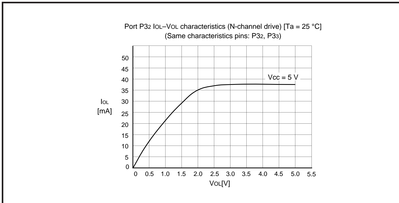
Fig. 19 N-channel open-drain output port N-channel side characteristics (Ta = 25 °C)
