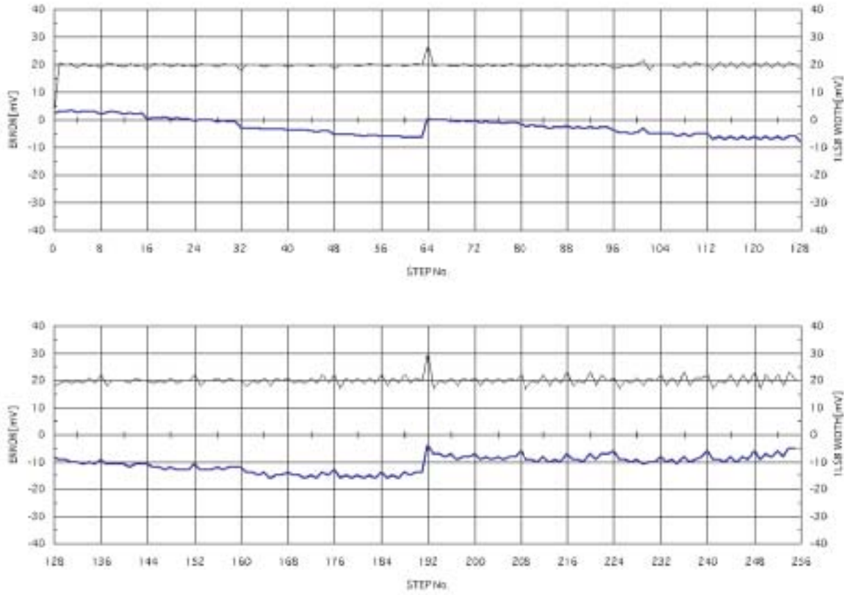
Fig. 33 Flash memory version D-A conversion standard characteristics
