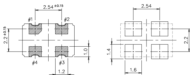
Recommended Soldering Pattern
