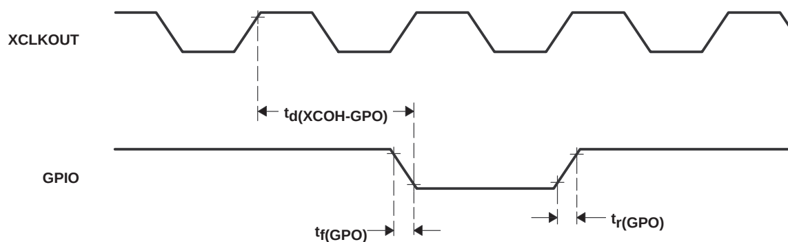
Figure 6-21. General-Purpose Output Timing
