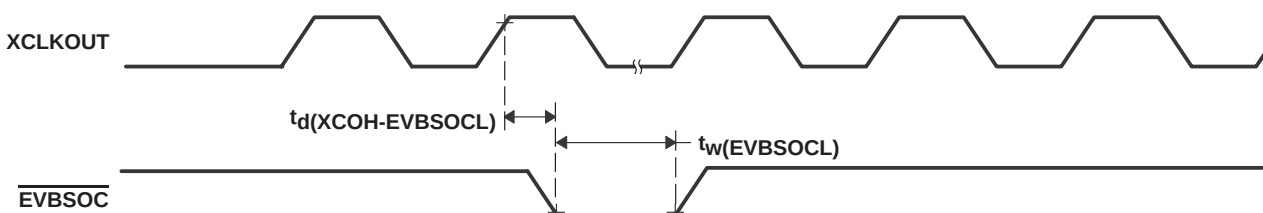
Figure 6–19. \overline{\text{EVBSOC}} Timing
