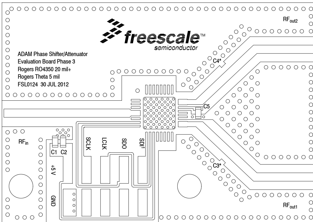
Figure 7. MMDS09254H Test Circuit Component Layout
