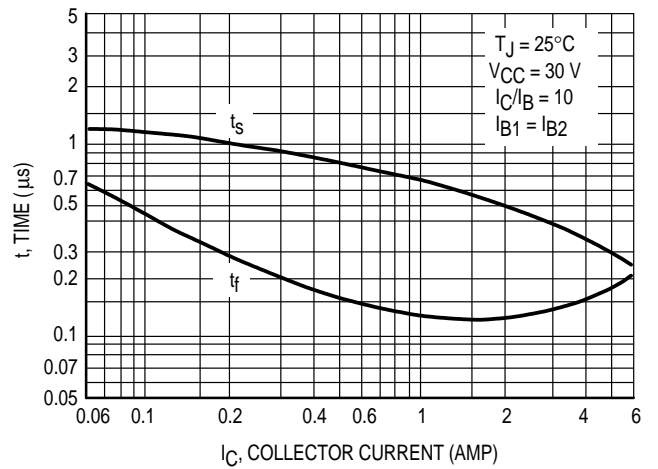
Figure 5. Turn-Off Time
