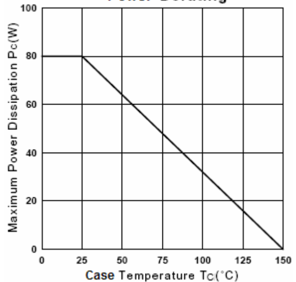
Power Derating
