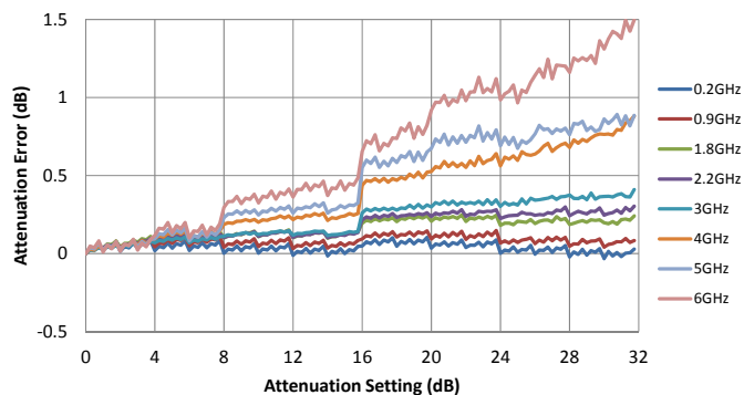
Figure 9. 0.25 dB Attenuation Error vs. Frequency
