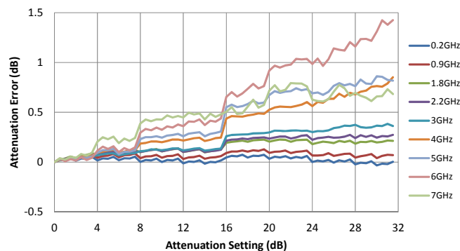
Figure 13. 0.5 dB Attenuation Error vs. Frequency
