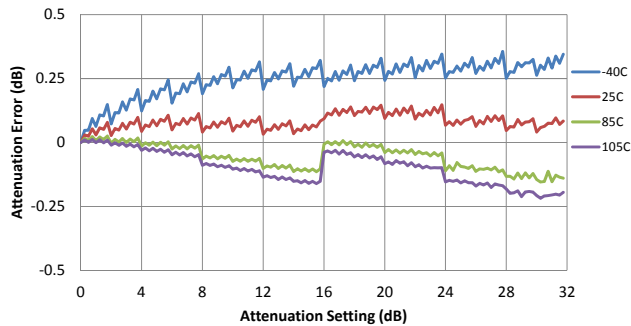
Figure 25. Attenuation Error @ 900 MHz vs. Temperature
