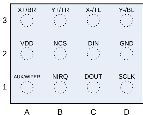
Figure 2. SX8653 WLCSP Top View, Solder Bumps on Bottom Side
