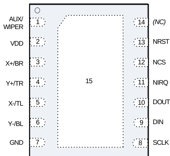
Figure 1. SX8653 DFN Top View, Pad on Bottom Side
