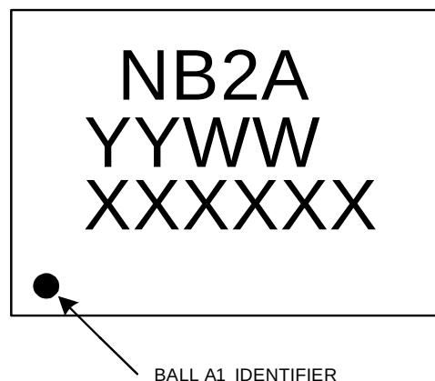
Figure 2. SX8653 WLCSP Top View, Solder Bumps on Bottom Side
