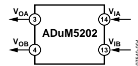
Figure 4. ADuM5202
