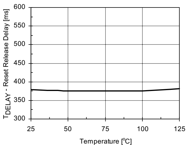
RESET Release Delay vs. Temperature
