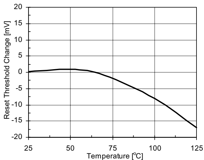
Threshold variation vs. Temperature
