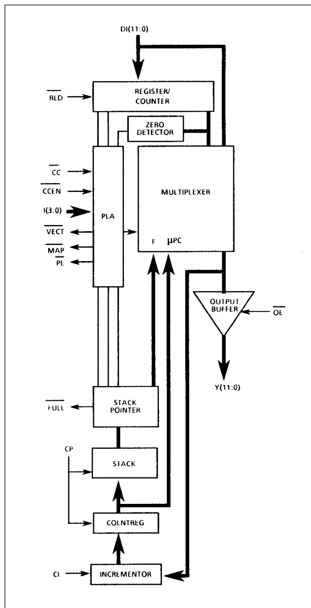
Figure 1: Block Diagram
