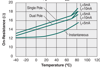
Typical On-Resistance vs. Temperature ( I_L=170\text{mA}_{DC} )
