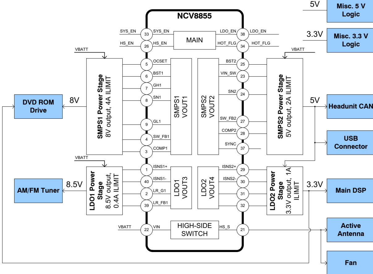
Figure 2. Automotive Radio System Block Diagram Example NCV8613B with NCV8855
