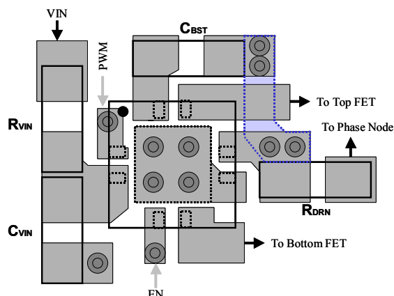
Fig. 13. Component placement for MLPQ-8.
