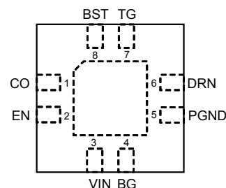
MLPQ-8 3x3mm Top View
