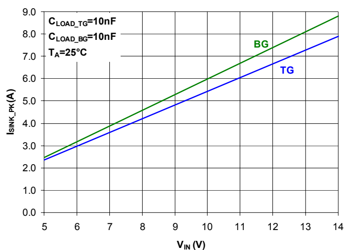
Fig. 10. Peak Sinking Current vs. Supply Voltage.
