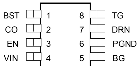
SOIC-8 Top View
