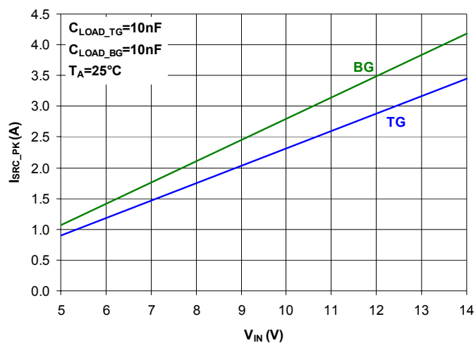
Fig. 9. Peak Sourcing Current vs. Supply Voltage.
