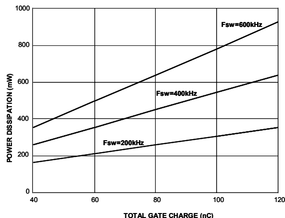
Fig. 11. Power dissipation.
