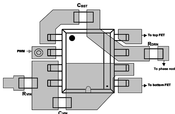
Fig. 12. Component placement for SOIC-8
