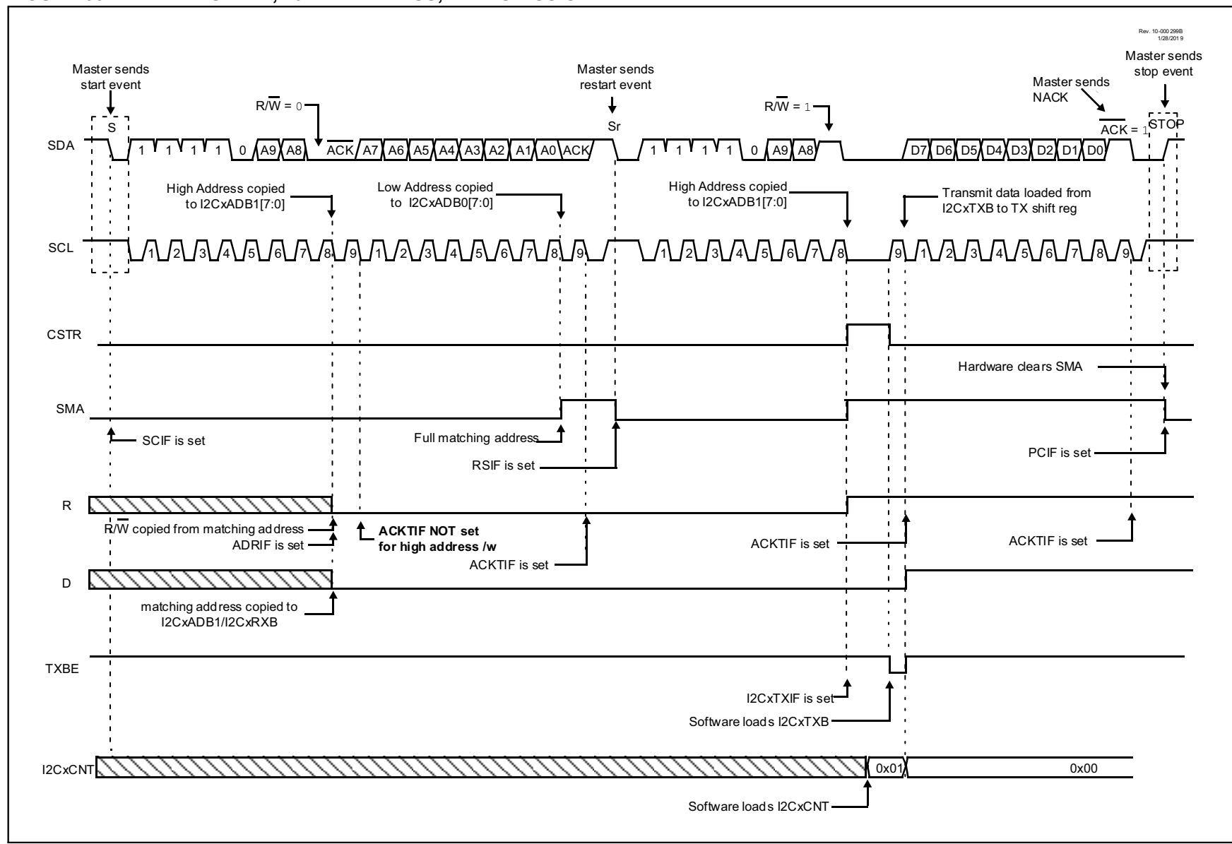
FIGURE 33-12: I 2 C SLAVE, 10-BIT ADDRESS, TRANSMISSION
