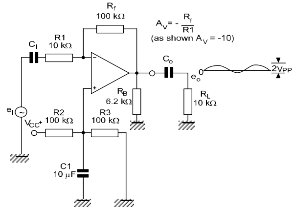
Figure 3: AC-coupled inverting amplifier
