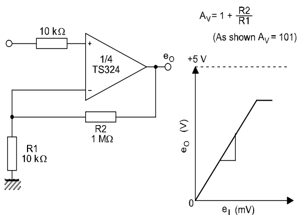
Figure 4: Non-inverting DC gain
