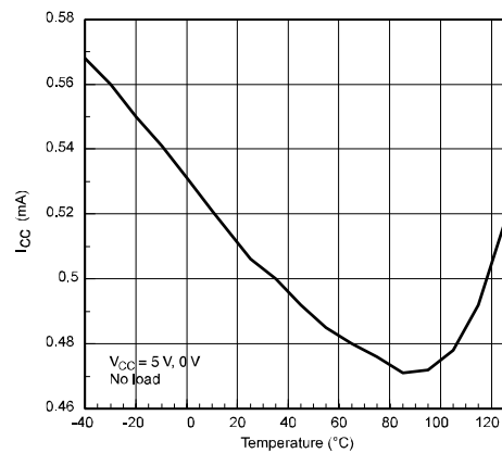
Figure 2: Current consumption versus temperature
