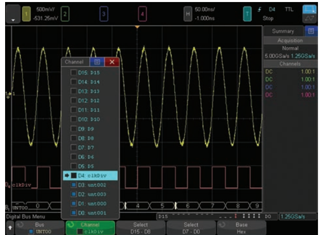
Figure 29. FPGA dynamic probe routing out internal FPGA signals, to be captured by the 4000 X-Series, correlated with this external analog sine wave in the design.
