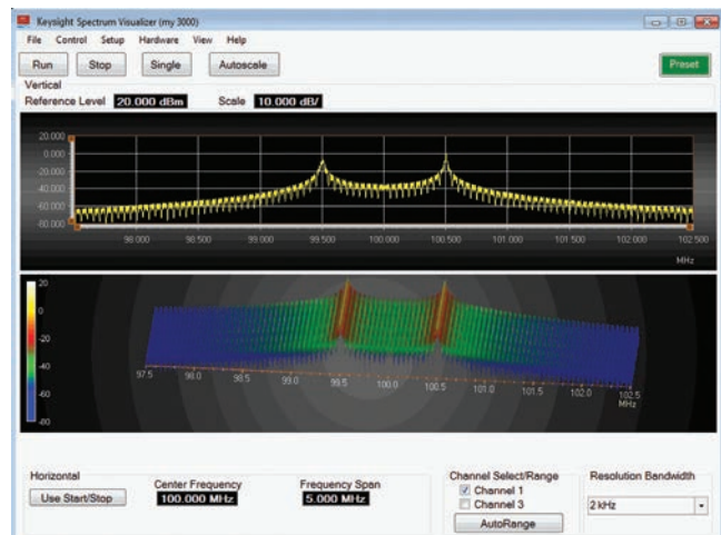
Figure 41. Waterfall view for KSV spectrogram measurements.
