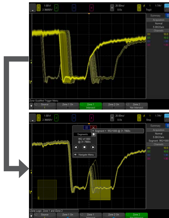
Figure 16. Combination of the InfiniiScan Zone touch trigger and segmented memory.
