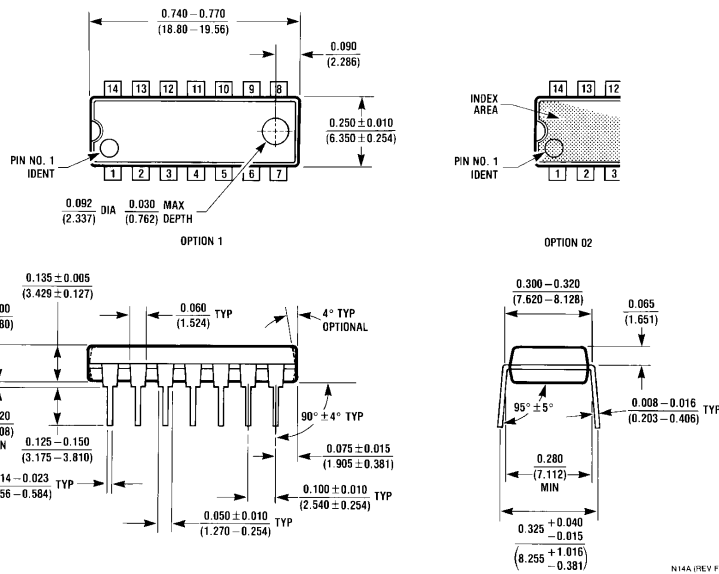
14-Pin Molded DIP Order Package Number LMC6044AIN or LMC6044IN NS Package Number N14A
