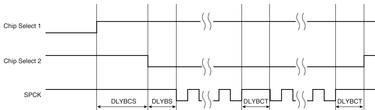
Figure 32-7. Programmable Delays
