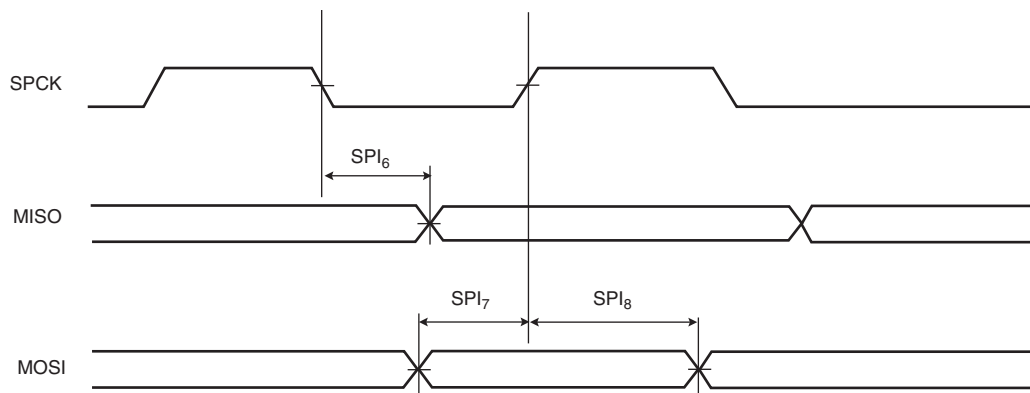
Figure 44-6. SPI Slave Mode with (CPOL=0 and NCPHA=1) or (CPOL=1 and NCPHA=0)
