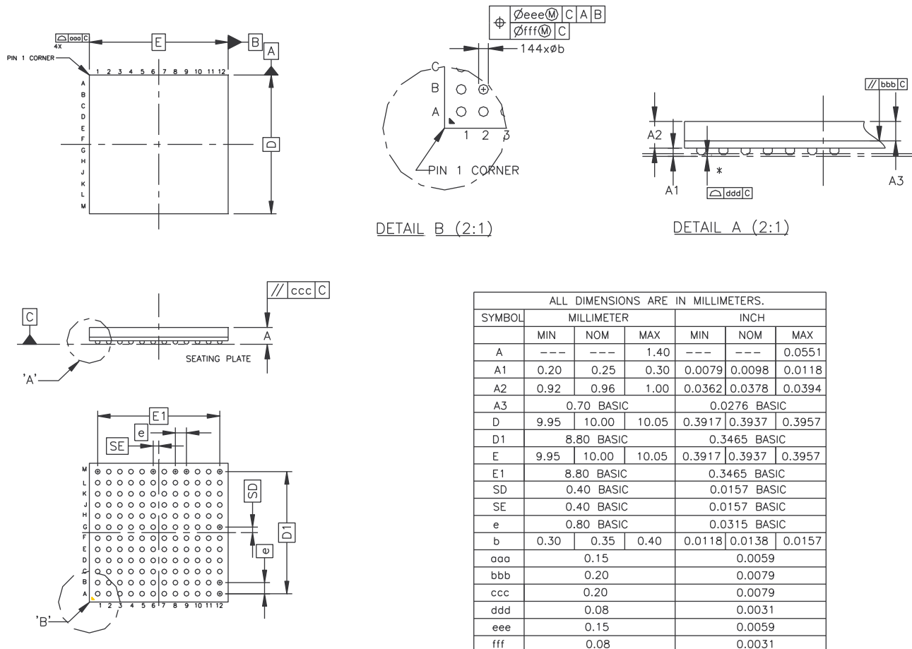
Figure 45-1. 144-ball BGA Package Drawing
