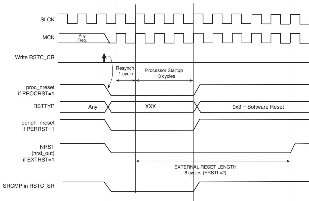
Figure 15-7. Software Reset
