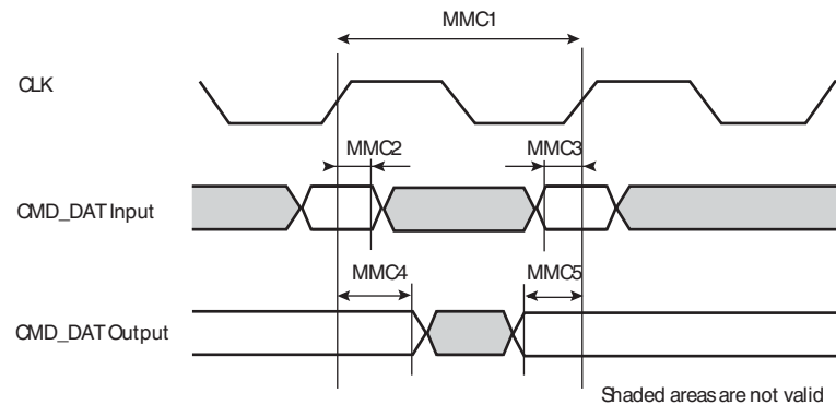
Figure 44-17. MMC Timings
