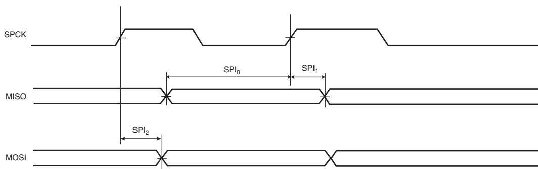
Figure 44-4. SPI Master Mode with (CPOL=0 and NCPHA=1) or (CPOL=1 and NCPHA=0)
