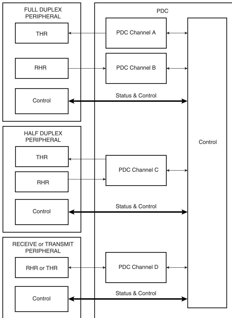
Figure 25-1. Block Diagram
