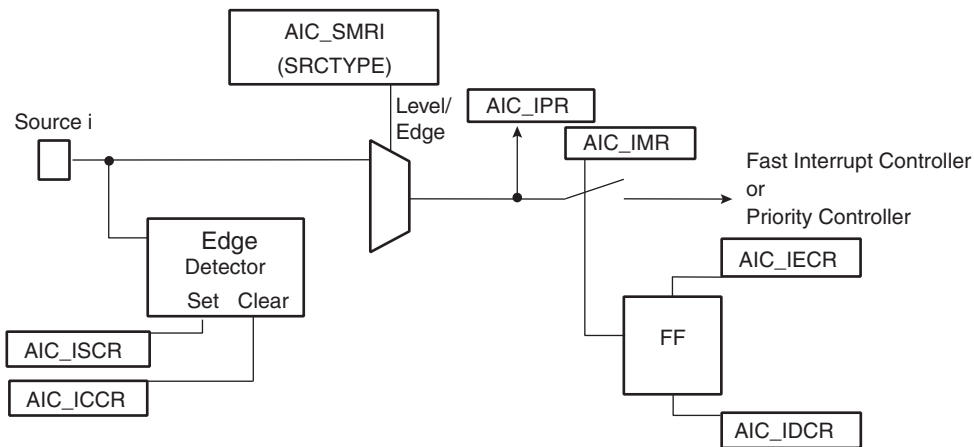
Figure 29-4. Internal Interrupt Source Input Stage
