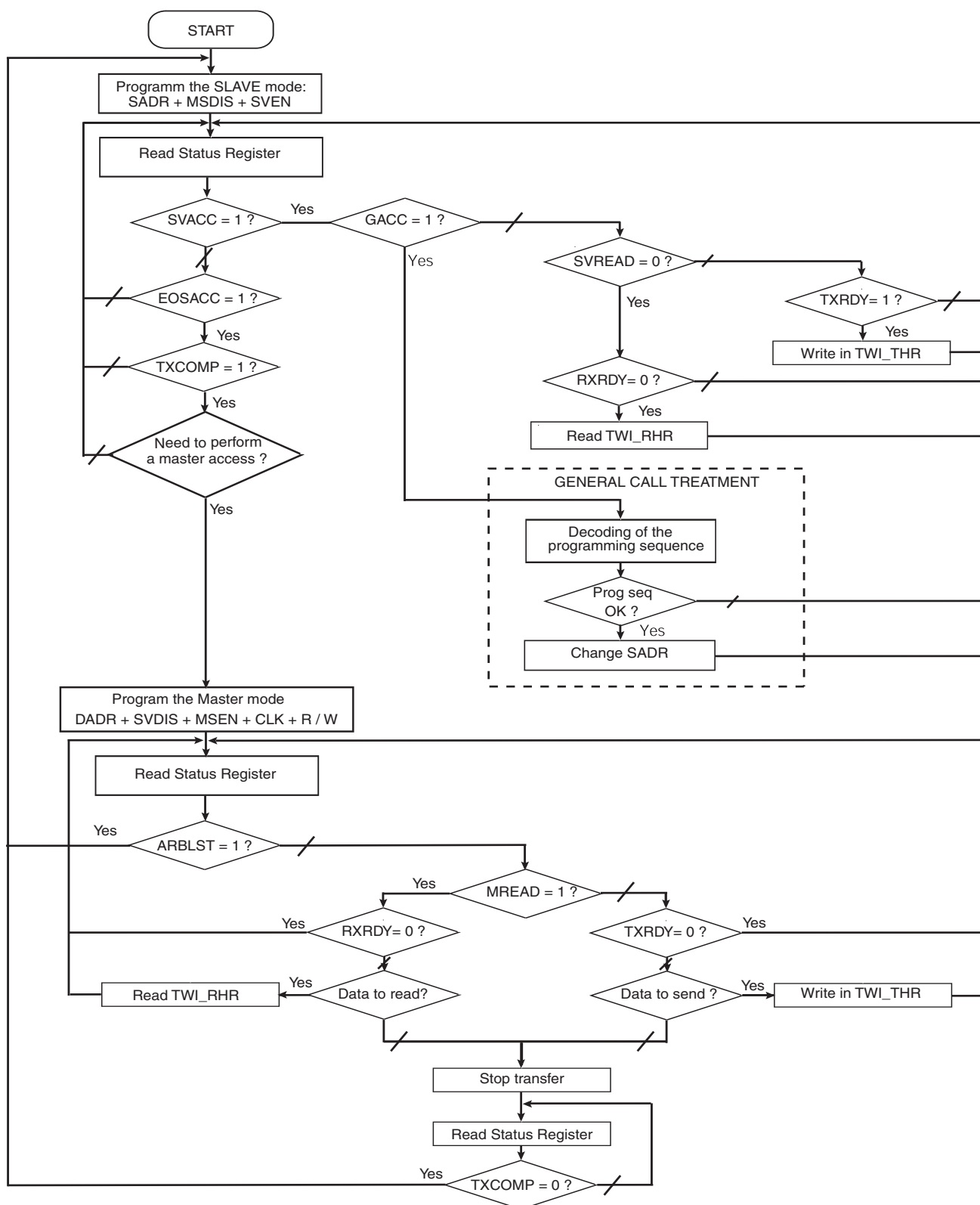
Figure 33-22. Multi-master Flowchart
