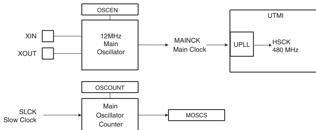
Figure 26-3. Main Oscillator Block Diagram
