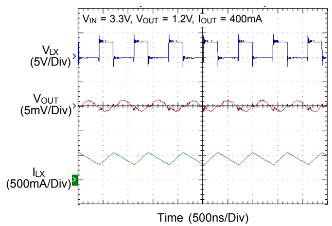
Output Ripple
