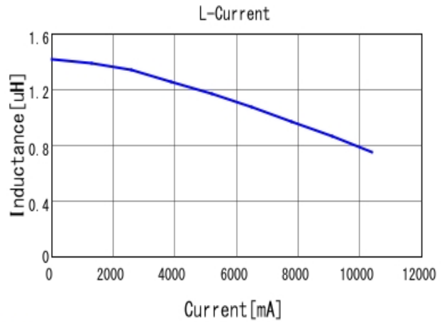
DFE322520FD-1R5M L-Current 20degC
