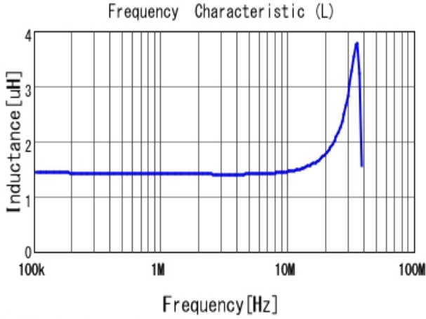
DFE322520FD-1R5M L
