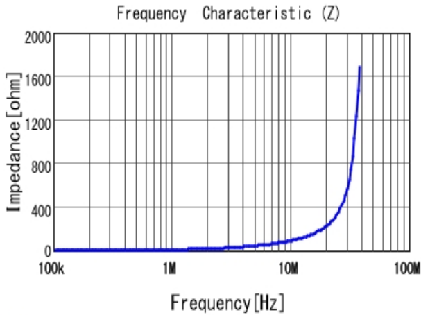
DFE322520FD-1R5M |Z|
