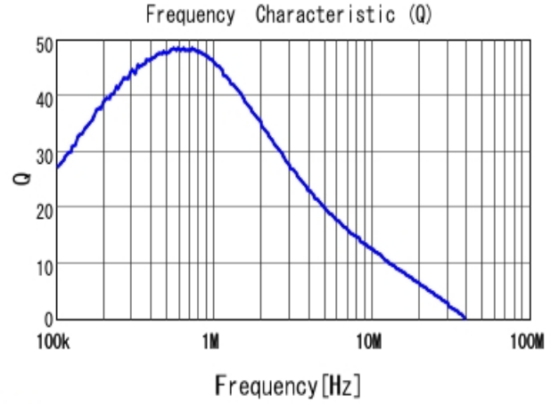
DFE322520FD-1R5M Q
