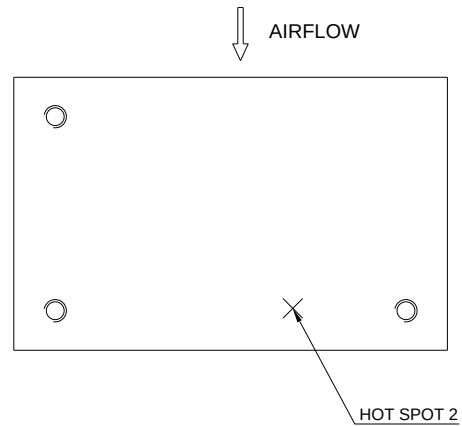
Figure 24: * Hot spot 2 temperature measured point. The allowed maximum hot spot 2 temperature is defined at 105 °C
