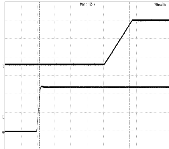
Figure 7: Turn-on transient at zero load current (20 ms/div). V_{in}=48V . Top Trace: V_{out} , 5V/div; Bottom Trace: input voltage, 20V/div
