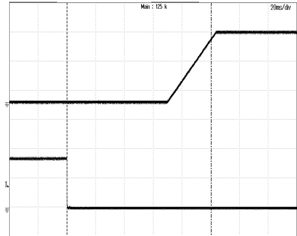
Figure 6: Turn-on transient at full rated load current (constant current load) (20 ms/div). V_{in}=48V . Top Trace: V_{out} , 5V/div; Bottom Trace: ON/OFF input, 2V/div
