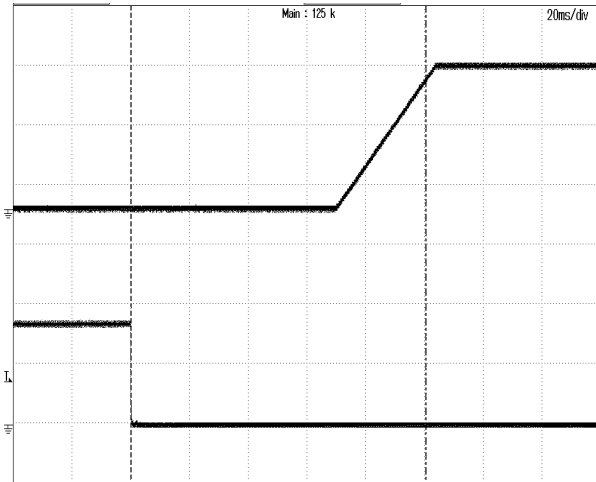
Figure 5: Turn-on transient at zero load current (20ms/div). V_{in}=48V . Top Trace: V_{out} , 5V/div; Bottom Trace: ON/OFF input, 2V/div
