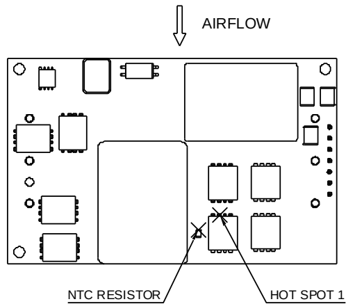
Figure 22: * Hot spot 1 & NTC resistor temperature measured points. the allowed maximum hot spot 1 temperature is defined at 118 °C
