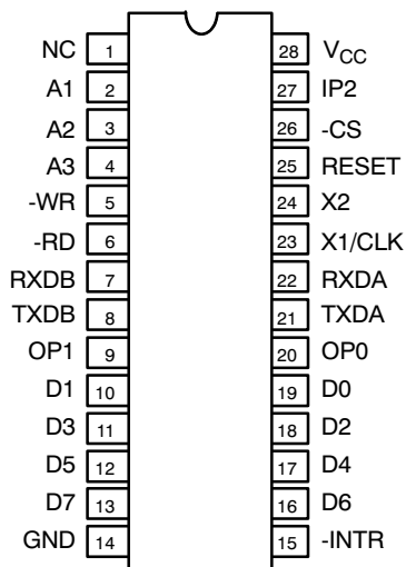
28 Lead PDIP (0.600")
