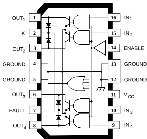
A2557xLB (SOIC)
