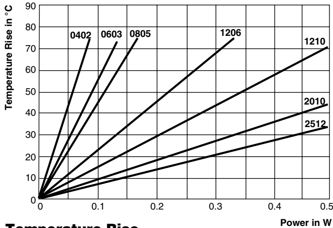
Temperature Rise
